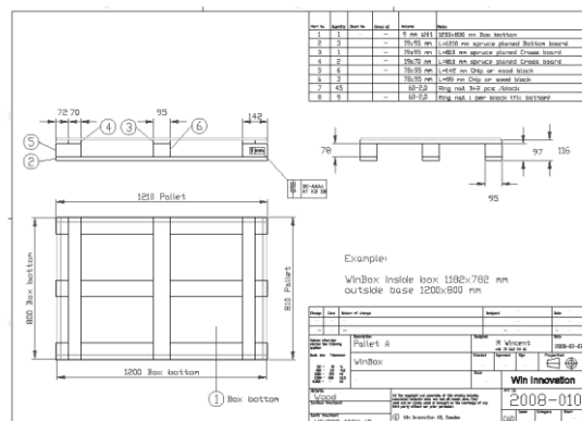
Drawing for pallet A nr. 2008-010
