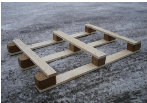
Pallet A for 4-ways handling
